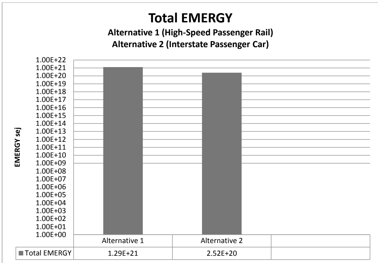
Figure 25. Total EMERGY
