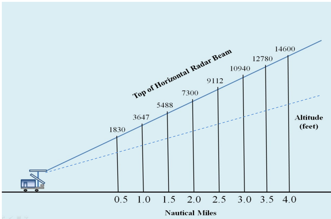
Figure 3. Vertical and Horizontal Beam Coverage (A; from DeText Inc. website 2013), and altitude coverage of the horizontal scanning radar (B), with the dashed line representing the center of the beam.
