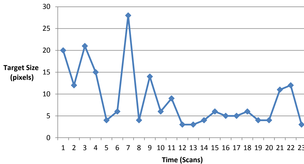
Figure 34. Scan to scan variation in radar estimates of target size for a red-tailed hawk at 0.6 NM. Over the course of 5 minutes, the hawk was tracked multiple times. Shown are consecutive target size estimates from several different tracks, totaling 23 scans.
